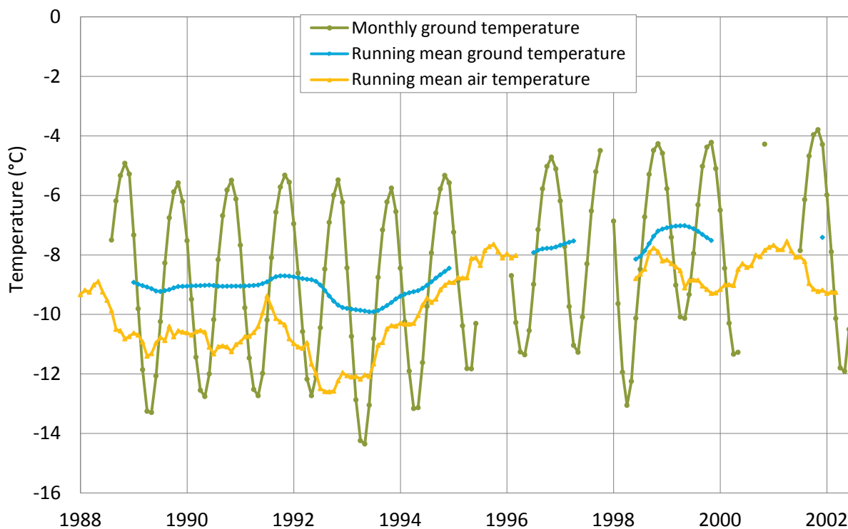
Figure 6. Monthly ground temperatures at a depth of 5 metres at Environment Canada's borehole at Iqaluit, 1988 to 2002.
