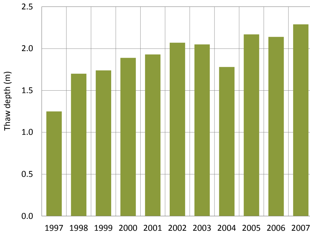
Figure 4. Maximum summer thaw depth for a site (BH4) at Baker Lake, 1997 to 2007. Source: adapted and updated from Smith et al. (2005b) and Throop et al. (2008)
