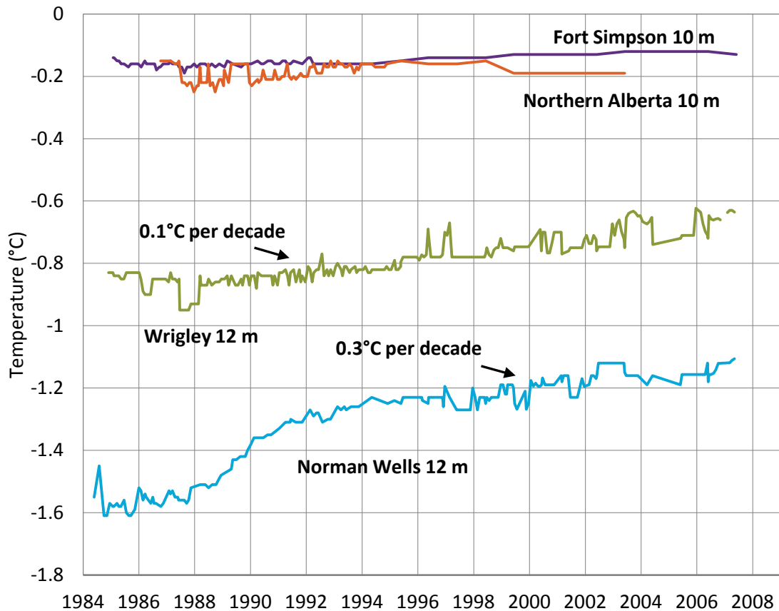
Figure 2. Ground temperatures between 1984 and 2007 at depths near 10 metres in the Mackenzie valley south of Norman Wells.
