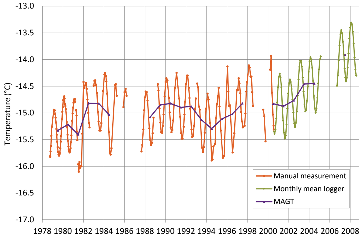
Figure 5. Observed and mean annual ground temperatures (MAGT) at a depth of 15 metres at Alert (BH5), 1978 to summer 2008.
