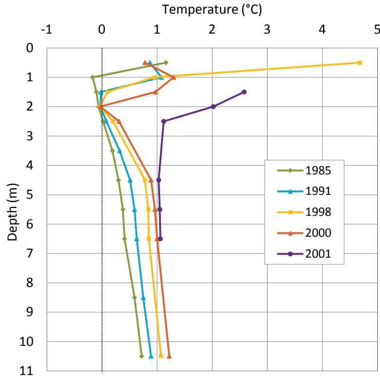
Figure 3. September ground temperature profiles between 1985 and 2001 for a site in a degrading peatland near Fort Simpson Northwest Territories. Source: adapted from Smith et al. (2008)
